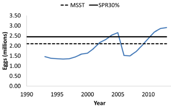
Figure 2. Red grouper SSB relative to MSST and MSY proxy 1993-2013
