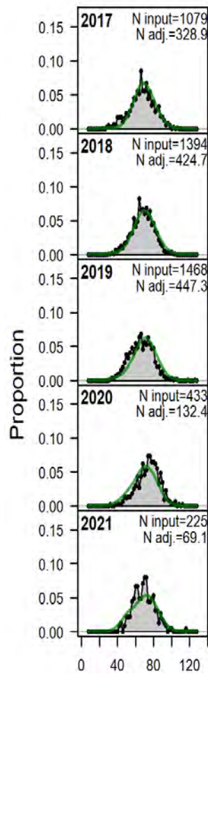
Figure 59 Continued. Observed and predicted length compositions for Gulf of Mexico Yellowedge Grouper in the Commercial Longline - East fishery for SEDAR 85 and SEDAR 22. Green lines represent predicted length compositions (red = female, blue = male, not fit to in SEDAR 85), while grey shaded regions represent observed length compositions. For SEDAR 85, 'N input' is the input sample size (number of length observations) and 'N adj.' is the sample size after adjustment by the Dirichlet-Multinomial parameter. For SEDAR 22, 'N adj.' is the input sample size ('N eff.' was not used).
