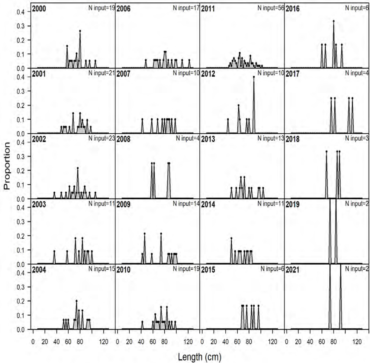
Figure 24. Observed length composition data of Gulf of Mexico Yellowedge Grouper from the NMFS Bottom Longline Survey - West. 'N input' is the number of length observations.
