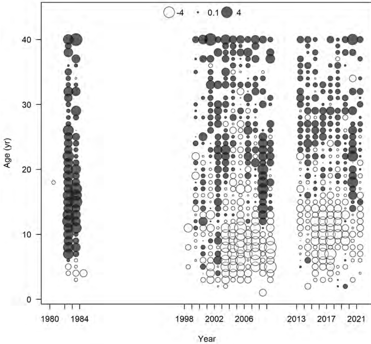
Figure 87. Pearson residuals for mean length-at-age of Gulf of Mexico Yellowedge Grouper landed by the Commercial Longline - East fleet. Closed bubbles are positive residuals (observed > expected) and open bubbles are negative residuals (observed < expected).
