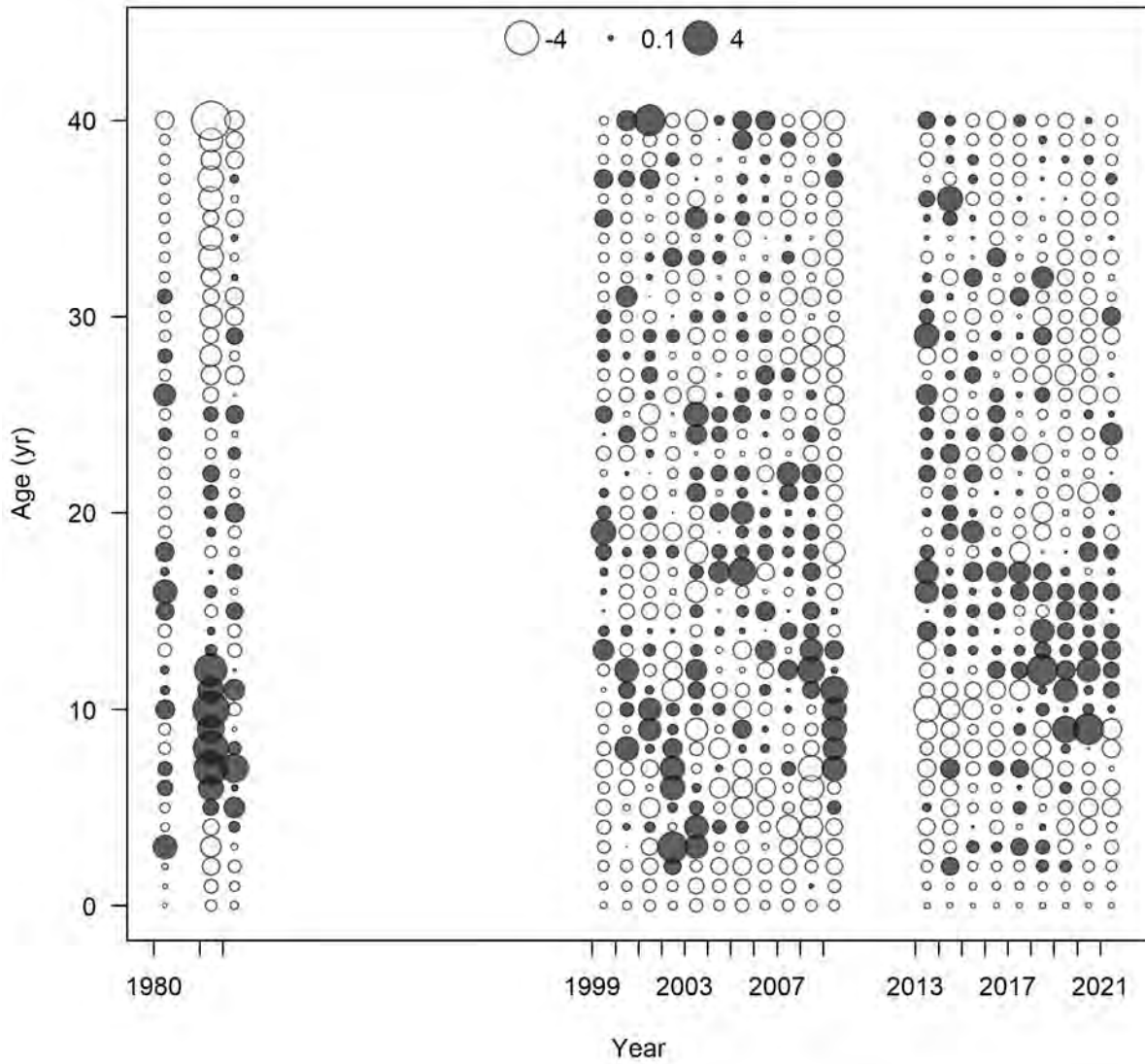
Figure 84. Pearson residuals for age compositions of Gulf of Mexico Yellowedge Grouper landed by the Commercial Longline - East fleet. Closed bubbles are positive residuals (observed > expected) and open bubbles are negative residuals (observed < expected).
