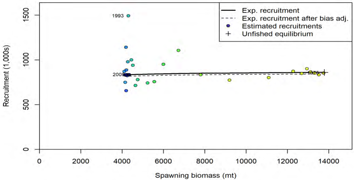
Figure 40. Predicted stock-recruitment relationship for Gulf of Mexico Yellowedge Grouper (steepness and \text{SigmaR} were fixed at 0.827 and 0.5, respectively). Plotted are predicted annual recruitments from Stock Synthesis (circles), expected recruitment from the stock-recruit relationship (black line), and bias adjusted recruitment from the stock-recruit relationship (dashed line).
