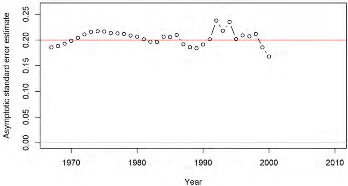
Figure 44. Asymptotic standard errors for recruitment deviations for Gulf of Mexico Yellowedge Grouper. The red line represents the fixed values of 0.5 and 0.2 used in the SEDAR 85 and SEDAR 22 models, respectively.
