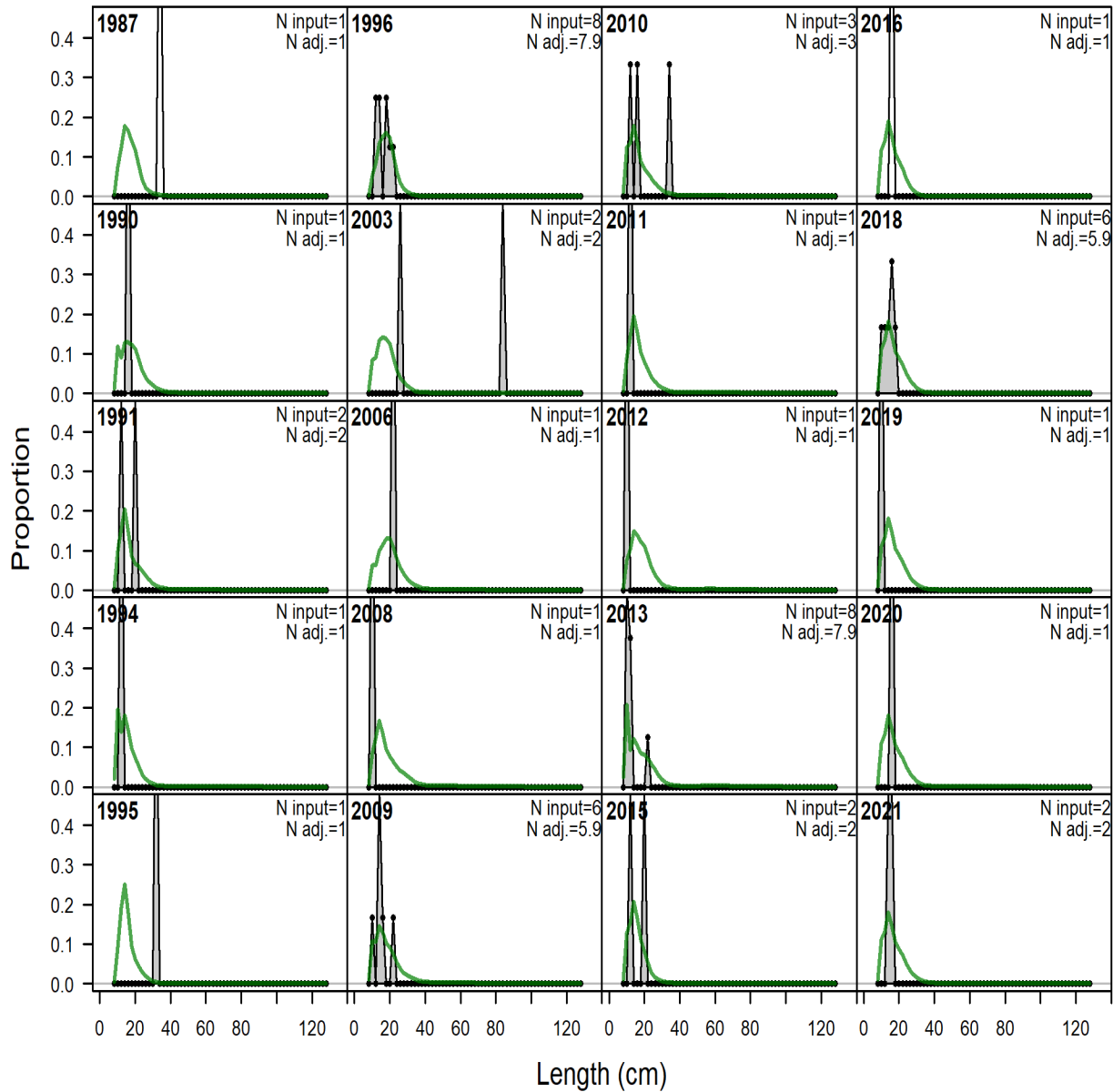
Figure 68. Observed and predicted length compositions for Gulf of Mexico Yellowedge Grouper caught in the NMFS/SEAMAP Groundfish Trawl Survey - East for SEDAR 85 and SEDAR 22. Green lines represent predicted length compositions (red = female, blue = male, not fit to in SEDAR 85), while grey shaded regions represent observed length compositions. For SEDAR 85, 'N input' is the input sample size (number of length observations) and 'N adj.' is the sample size after adjustment by the Dirichlet-Multinomial parameter. For SEDAR 22, 'N adj.' is the input sample size ('N eff.' was not used).
