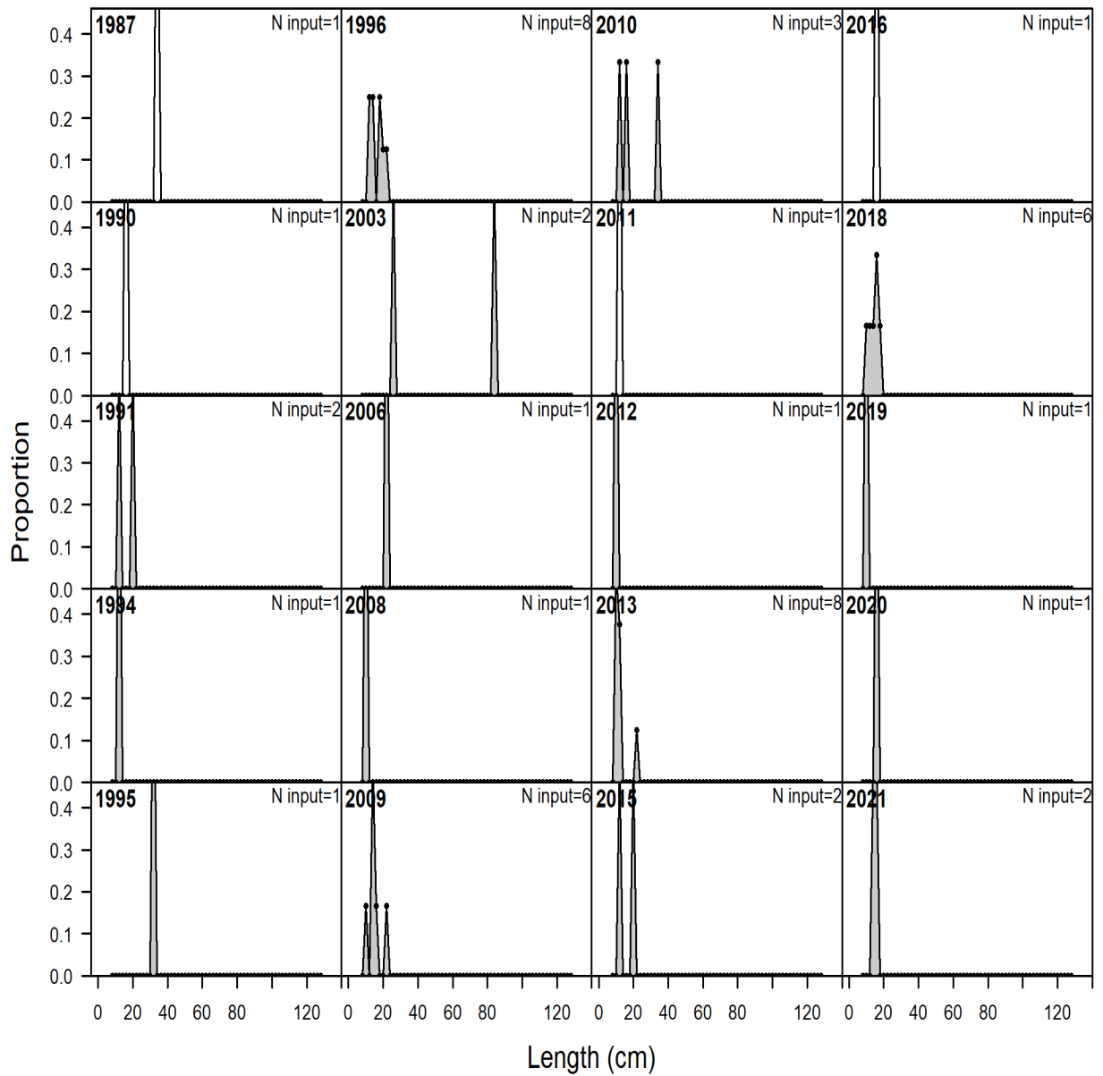
Figure 28. Observed length composition data of Gulf of Mexico Yellowedge Grouper from the NMFS/SEAMAP Groundfish Trawl Survey - East. 'N input' is the number of length observations.
