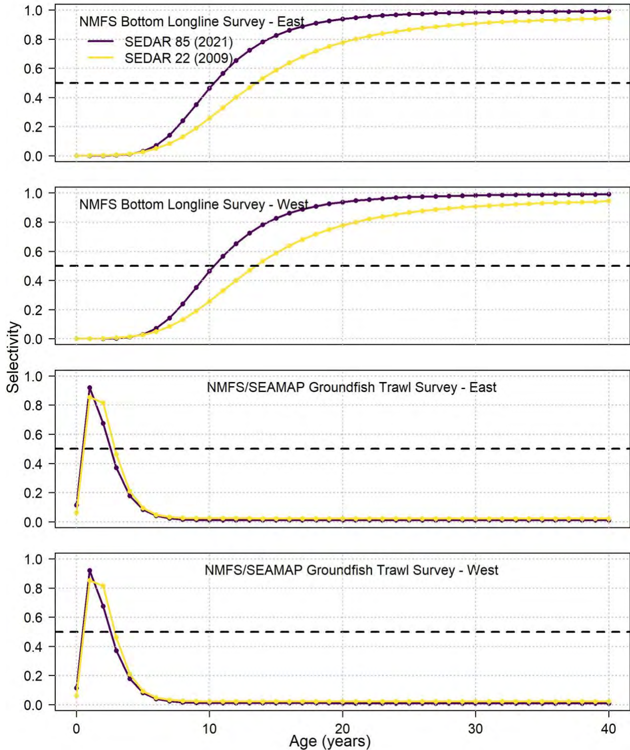
Figure 39. Derived age-based selectivity for each survey for Gulf of Mexico Yellowedge Grouper in the terminal year of each assessment (given in parentheses). Dashed horizontal line indicates 50%.
