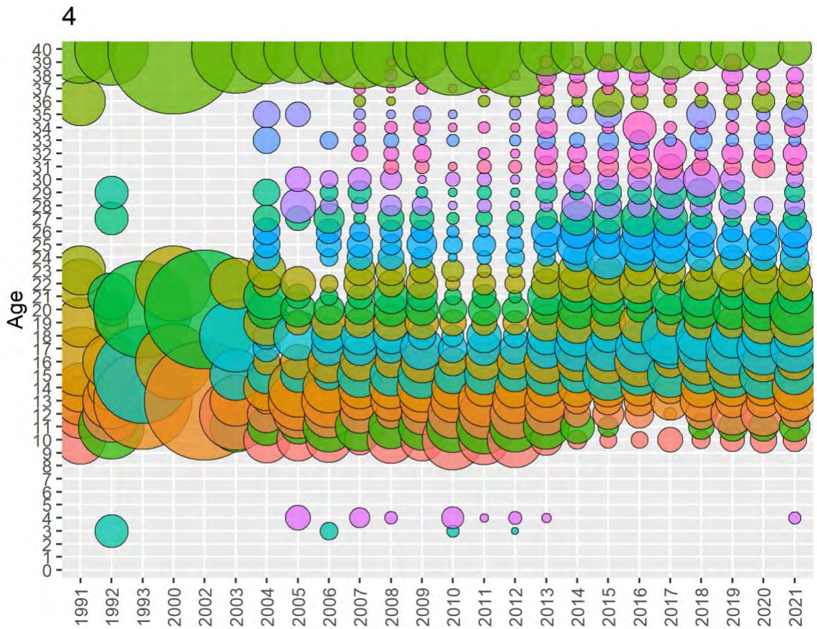
Figure 19. Observed relative age proportions (bubbles) in each year for Gulf of Mexico Yellowedge Grouper in the Commercial Longline - West fishery. The histogram shows annual sample sizes. All years of available data are shown before data exclusions.
