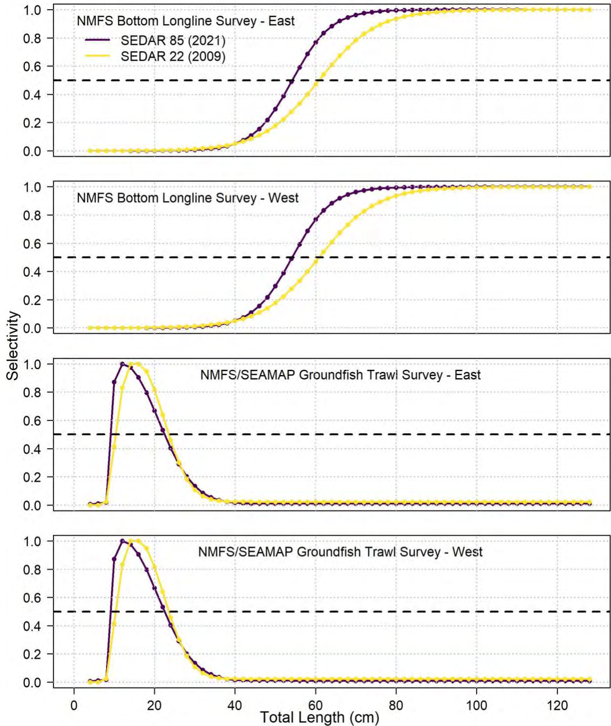
Figure 38. Length-based selectivity for each survey for Gulf of Mexico Yellowedge Grouper in the terminal year of each assessment (given in parentheses). Dashed horizontal line indicates 50%.
