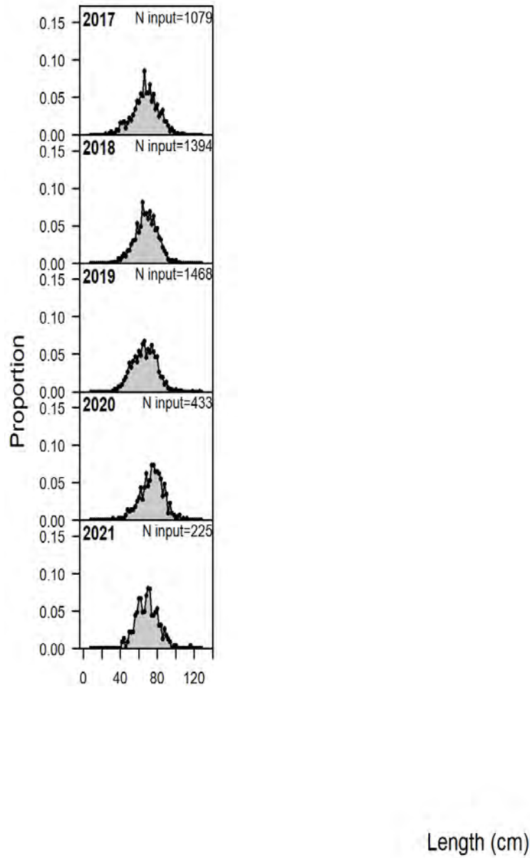
Figure 13 Continued. Observed length composition of Gulf of Mexico Yellowedge Grouper in the Commercial Longline - East fishery. 'N input' is the number of length observations.
