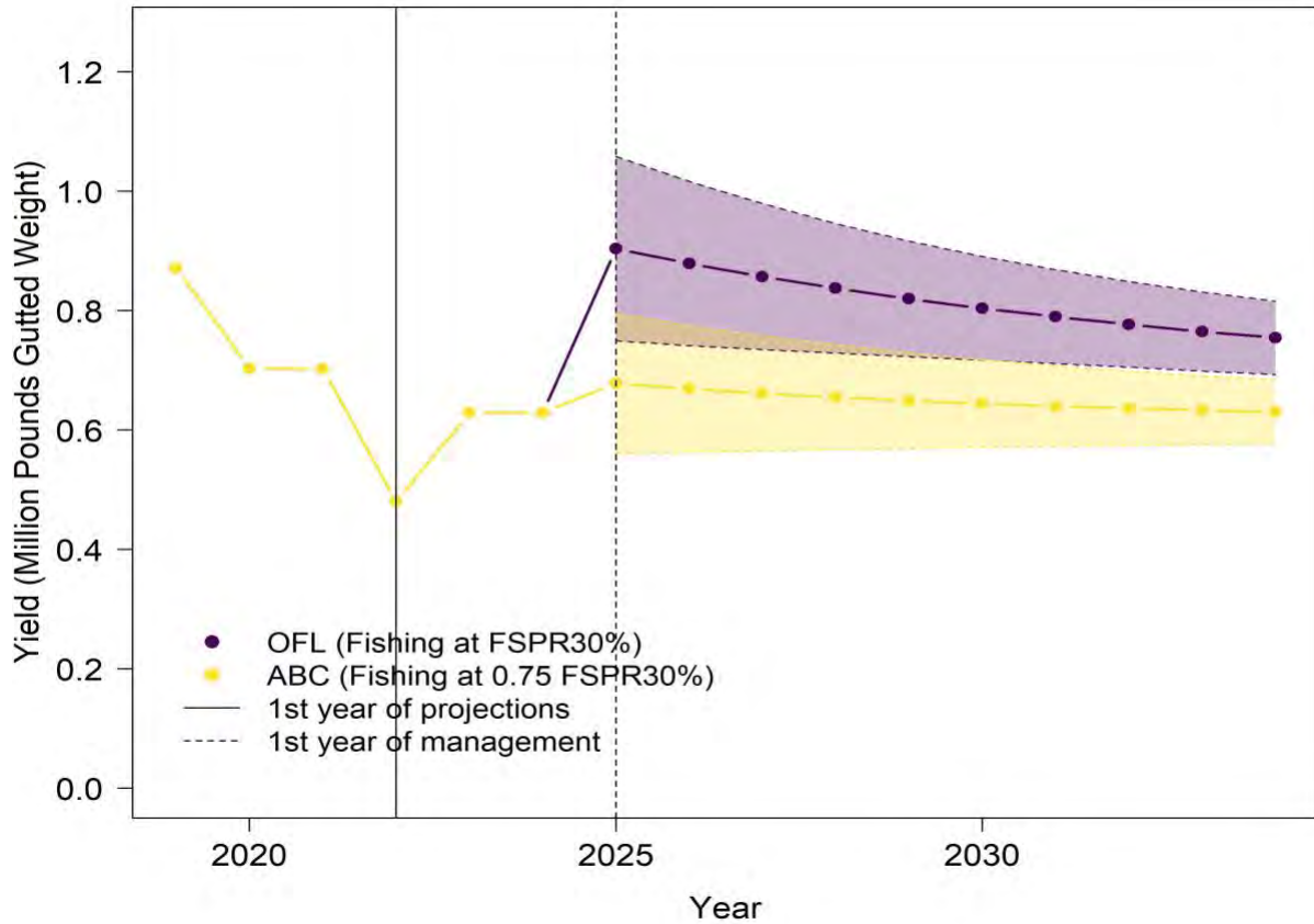
Figure 125. Historic (2019-2021), interim (2022-2024) and forecasted yields (2025+) for the OFL (fishing set at F_{30\%SPR} ) and ABC (directed F = 0.75 \times Directed F at F_{30\%SPR} (0.061)) projections for Gulf of Mexico Yellowedge Grouper with recruitment predicted by the stock-recruit curve from 2013 throughout the projection period . An SPR proxy of 30% was specified in the SEDAR 85 Terms of Reference.
