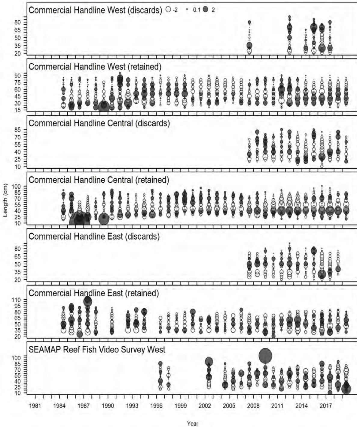
Figure 146. Pearson residuals for discard and retained length composition data by year compared across fleets and surveys for Gulf of Mexico Red Snapper for SEDAR 74. Closed bubbles are positive residuals (observed > expected) and open bubbles are negative residuals (observed < expected).
