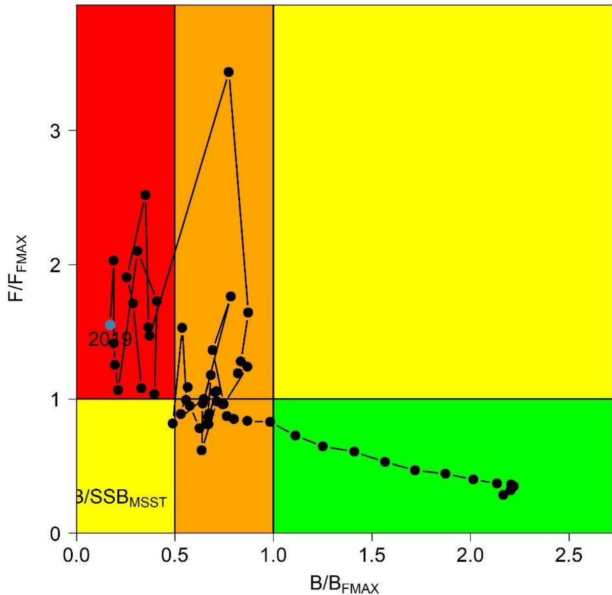
Figure 132. Kobe plot illustrating the trajectory of stock status. The orange coloring indicates regions where the stock is below the biomass target but above the biomass threshold ( MSST = 0.5 \times SSB_{FMAX} ). The 2019 terminal year stock status is indicated by the gray dot. See Table 33 for specifics on the years above F/F_{MAX}=1 and below B/B_{MSST}<0.5 . Annual exploitation rates used to calculate F/F_{MAX} include red tide F from the bycatch-only fleet. SSB defined as SSB combined.
