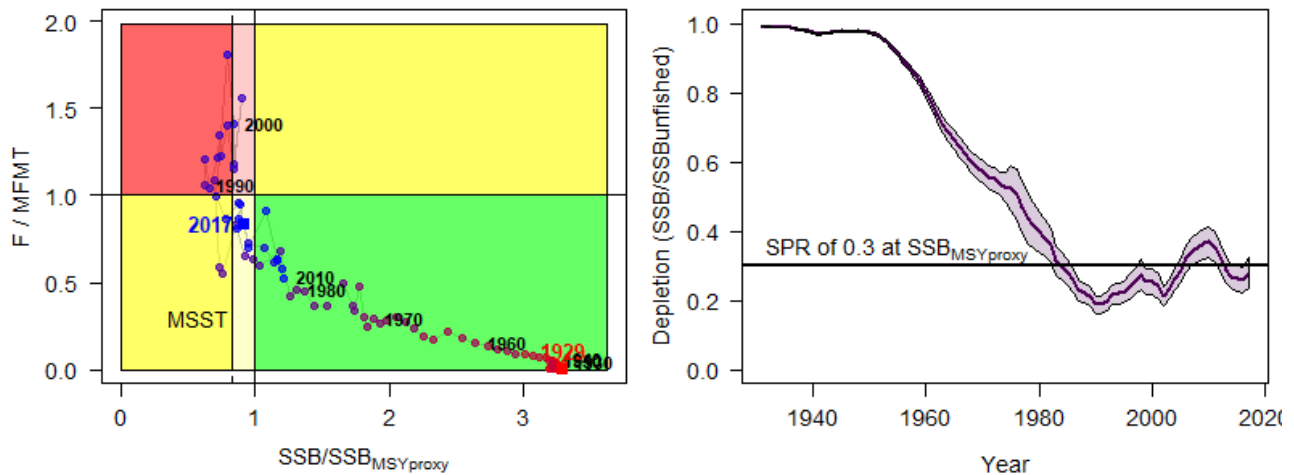
Figure 1: Kobe plot showing the progression of exploitation status for Gulf King Mackerel from 1929 to 2017, with the Minimum Stock Size Threshold (MSST) denoted [left panel]. Each point reflects a single year, labels are specified every 10 years, and colors gradually change from red (1929) through purple and ultimately blue (2017). Stock depletion with 95% asymptotic confidence intervals (shaded region) [right panel].
